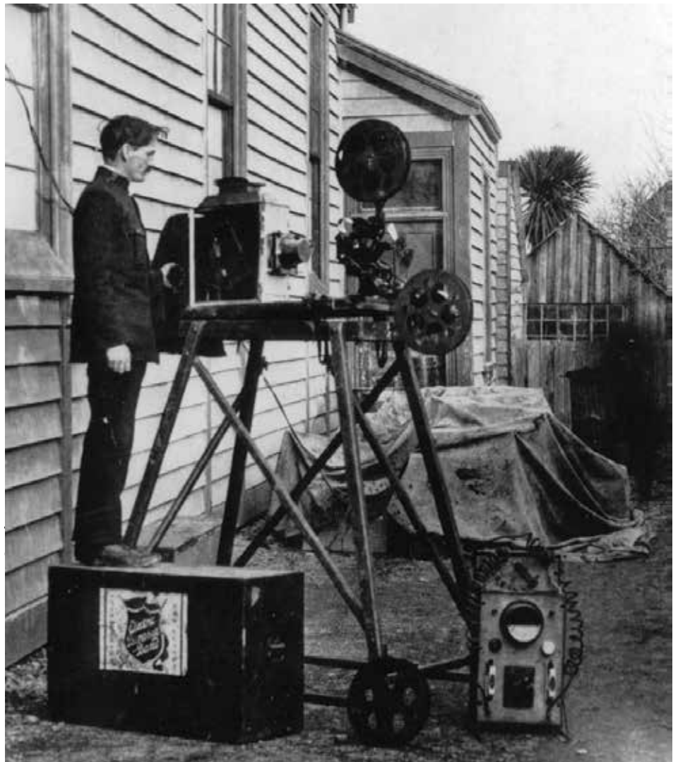
Early Gaumont projector used by The Salvation Army Limelight Department (Image courtesy of the Alexander Turnbull Library.)
